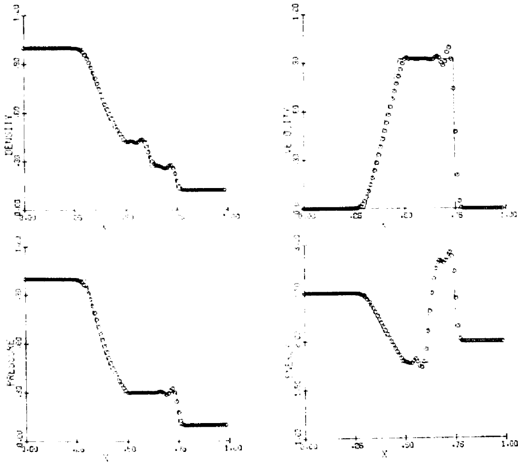
FIG. 7. MacCormack's method.
