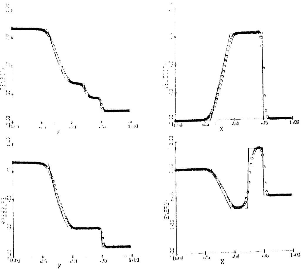
FIG. 13. Hybrid method.
