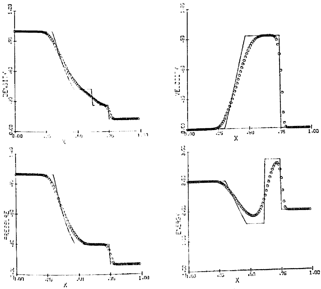
FIG. 8. Rusanov's first-order method.
