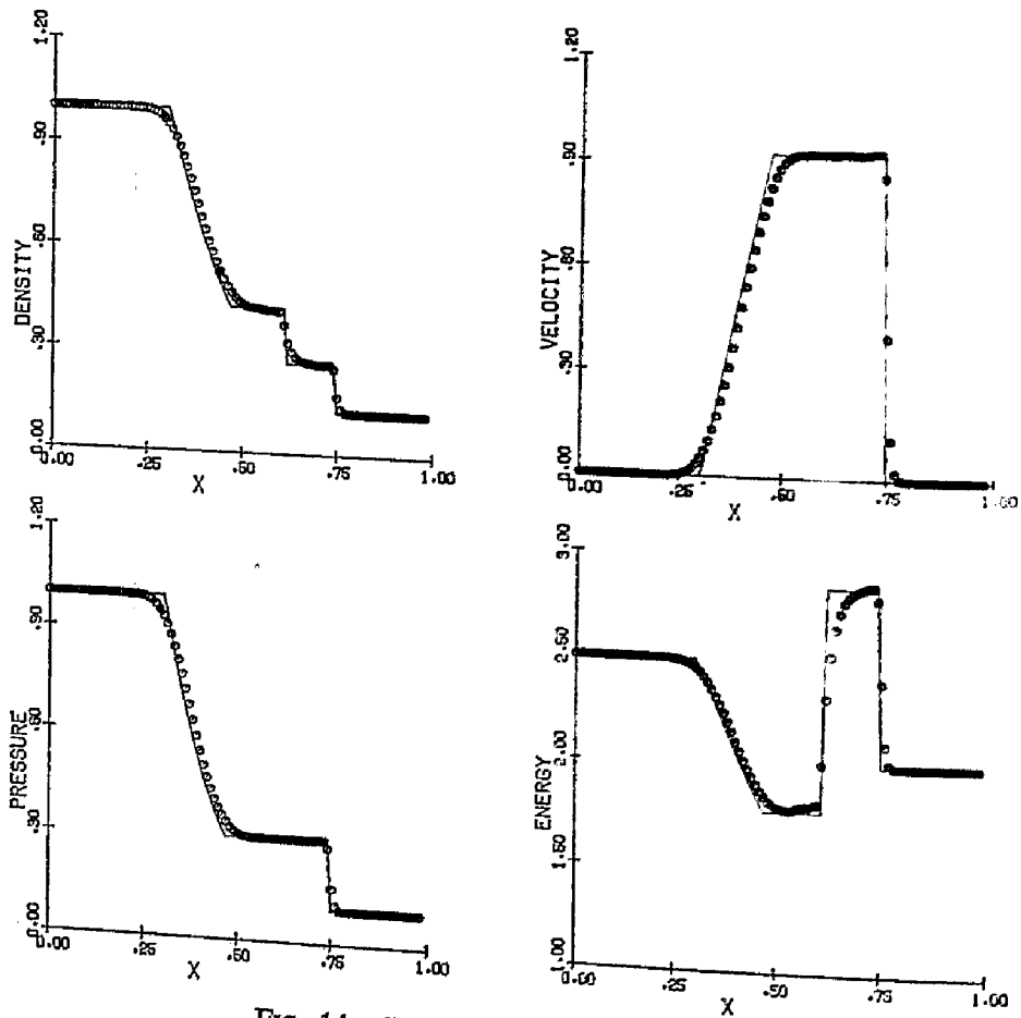
FIG. 14. Hybrid method with ACM.
