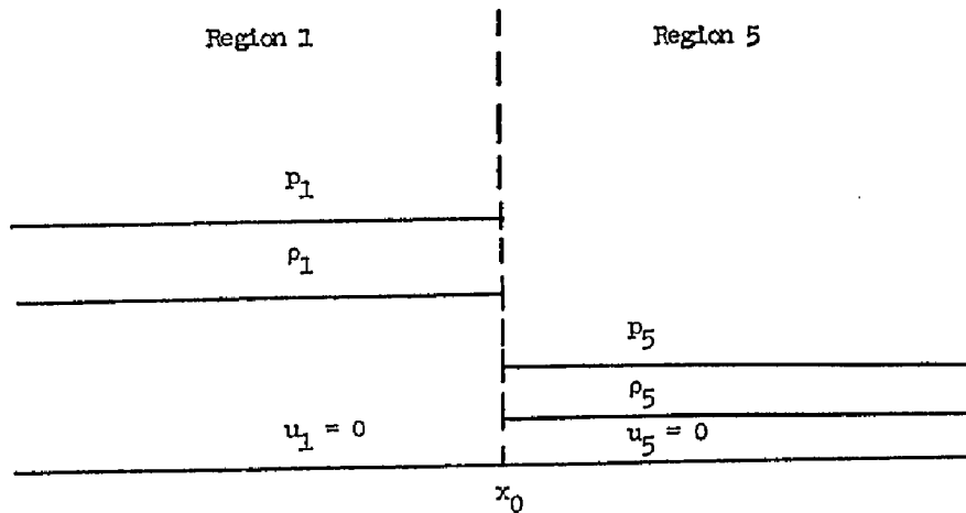
FIG. 2. Shock tube at t = 0 .
