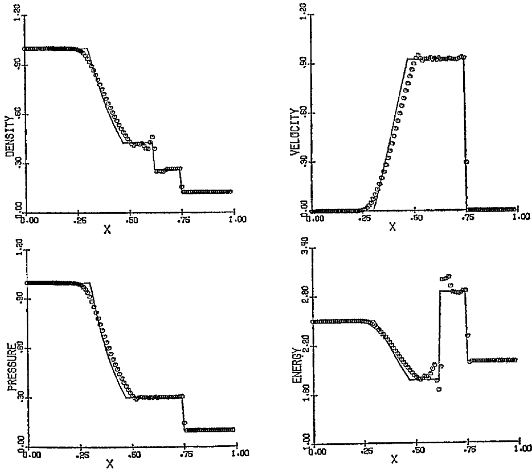
FIG. 5. Godunov's method with ACM.
