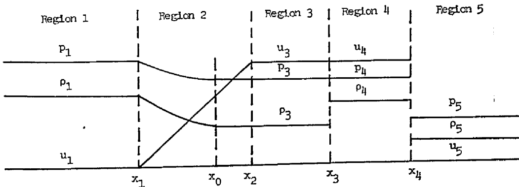
FIG. 3. Shock tube at t > 0 .
