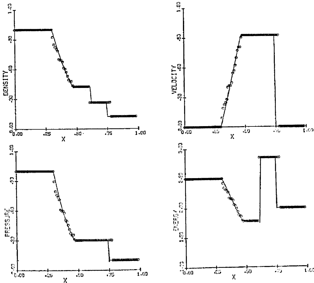
FIG. 11. Glimm's method.
