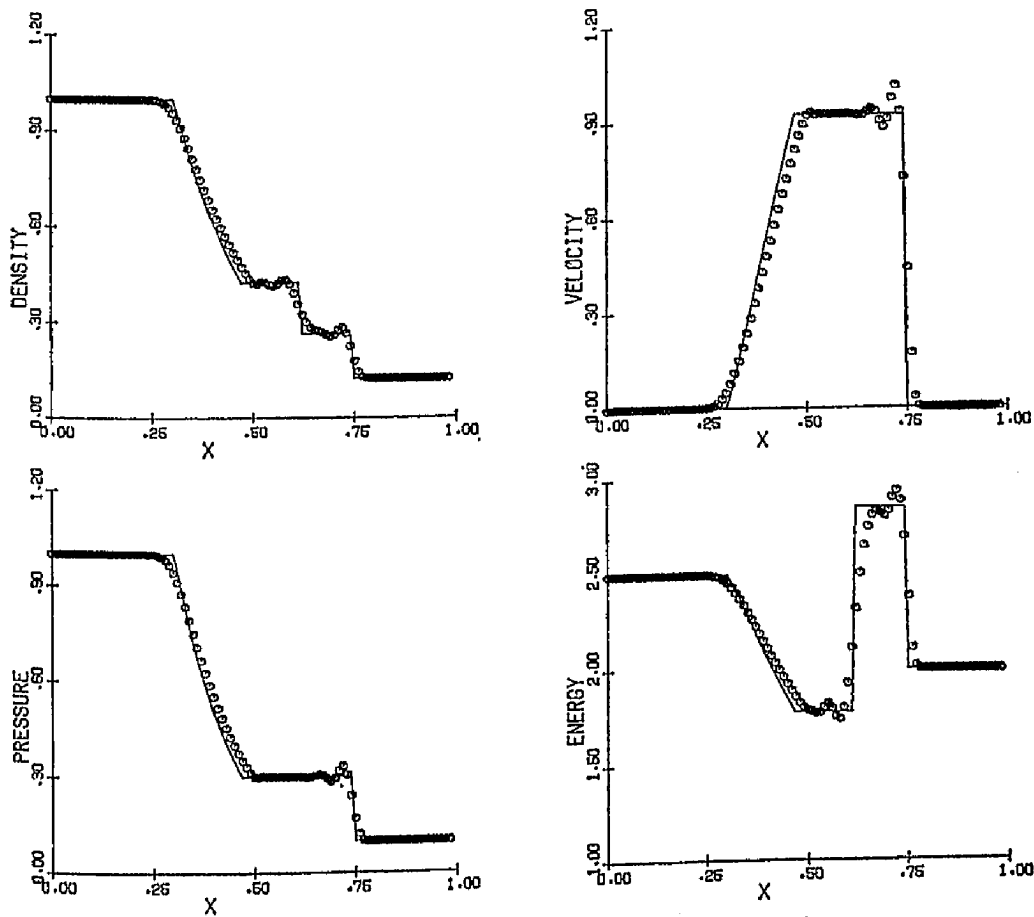
FIG. 6. Two-step Lax-Wendroff method.
