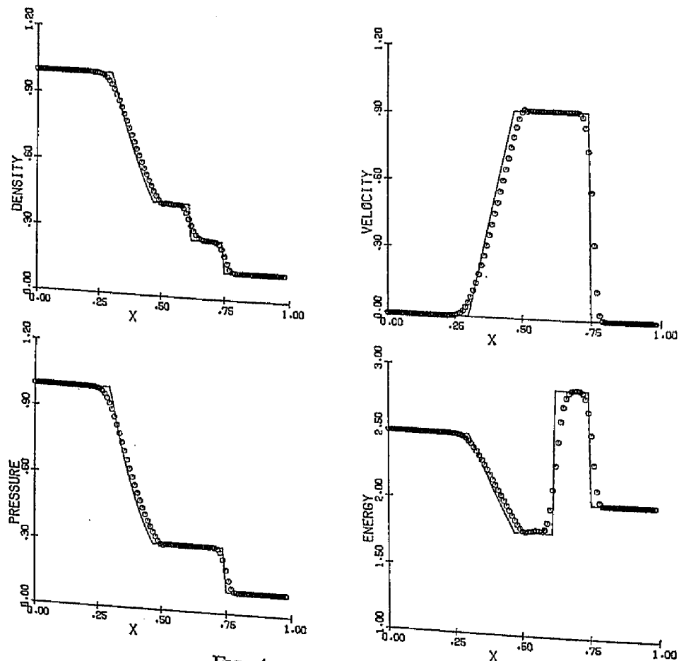
FIG. 4. Godunov's method.
